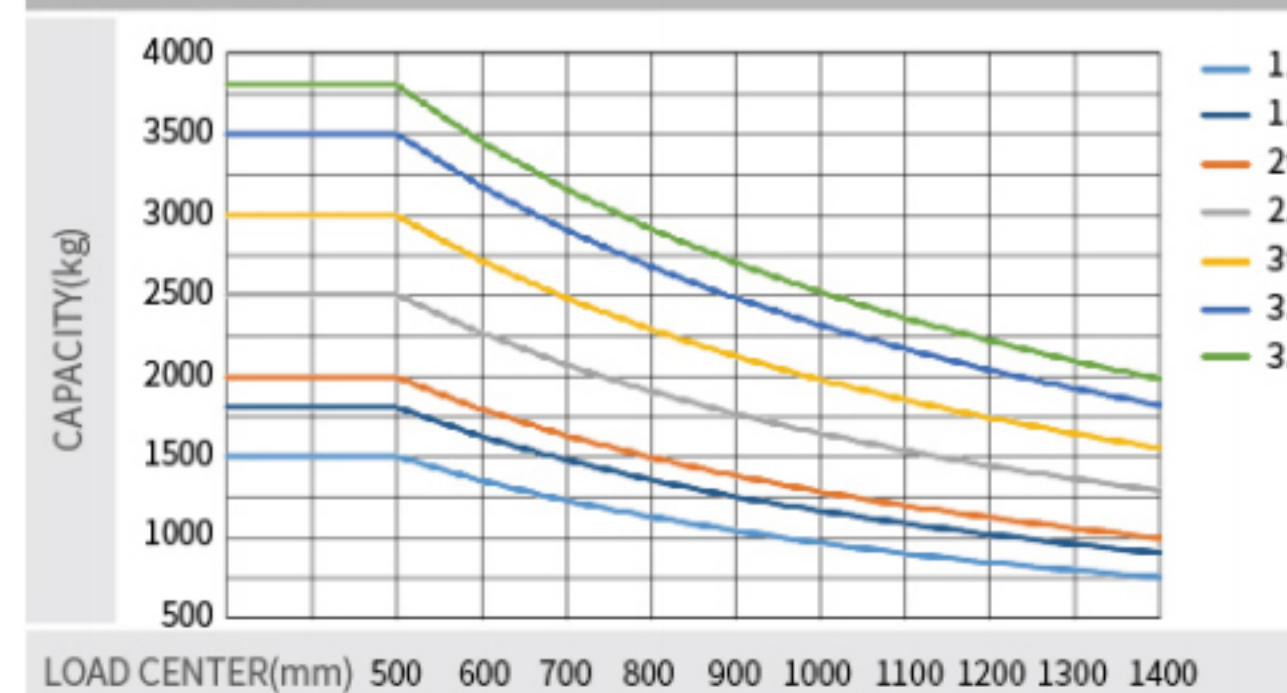
Load curve
