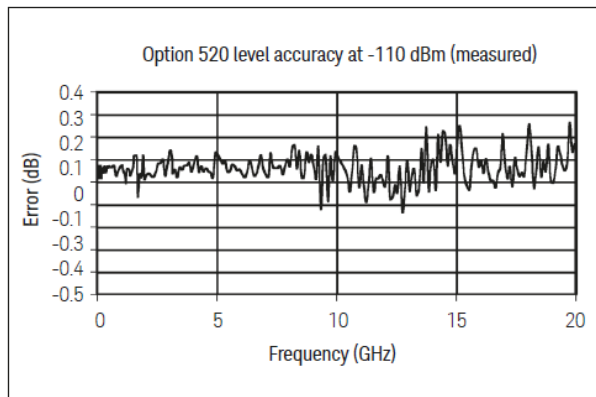
Level accuracy (measured)
