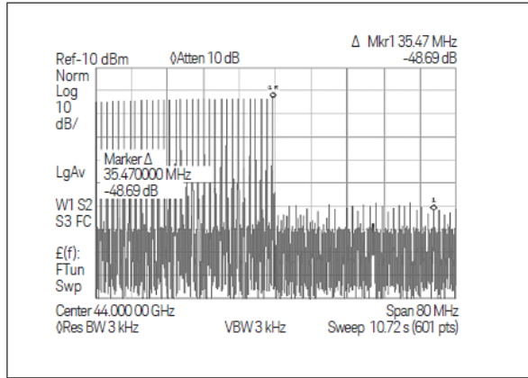
44 GHz image rejection (measured)
