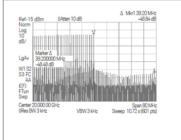
20 GHz image rejection (measured)
