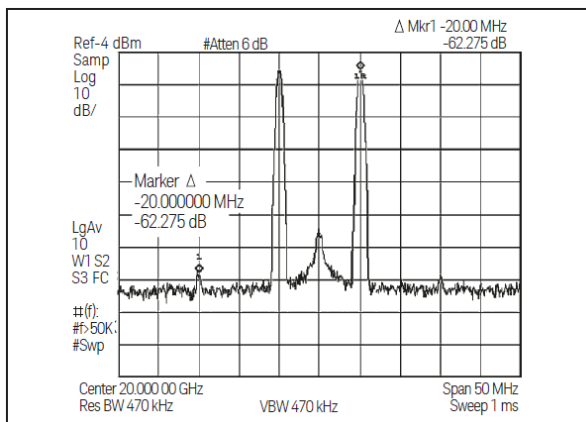
20 GHz two-tone (measured)
