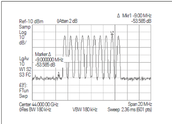
44 GHz multitone (measured)
