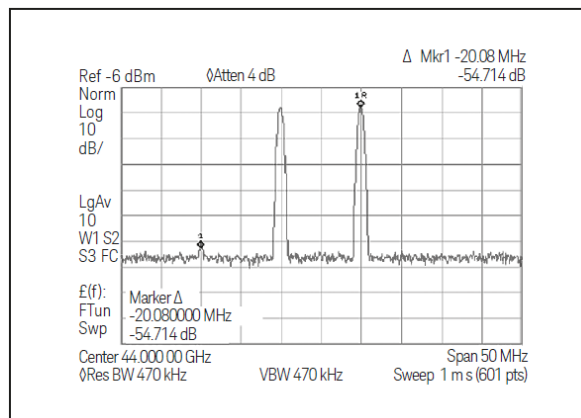
44 GHz two-tone (measured)
