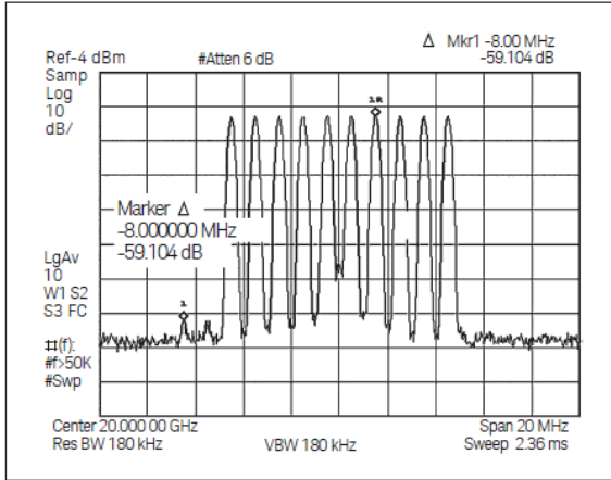
20 GHz multitone (measured)
