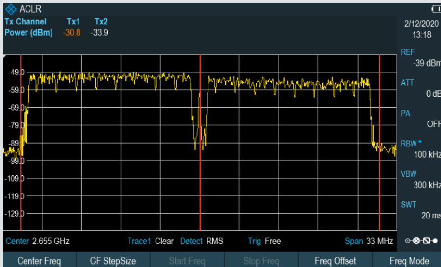
Gated trigger in ACLR mode with advanced the R&S®ZPH-K57 advanced gated trigger measurements option
