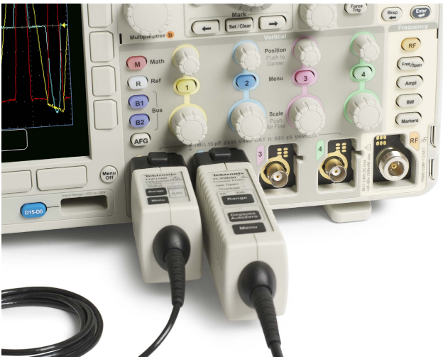
TekVPI probe interface simplifies connecting your probes to the oscilloscope.
