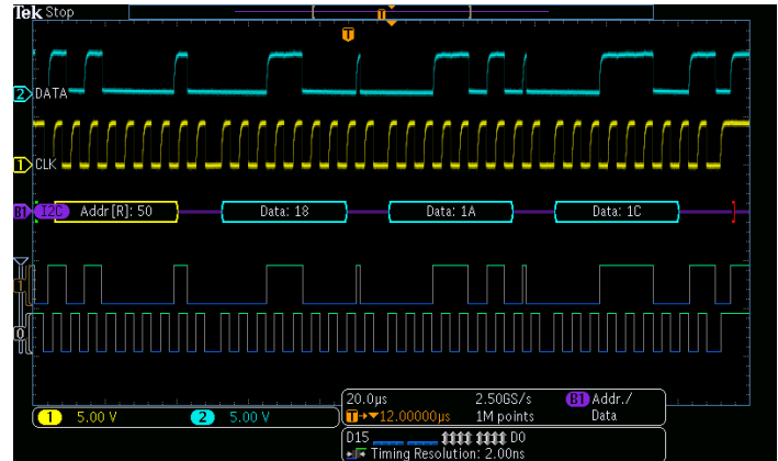
Triggering on a specific address and data packet going across an I 2 C bus. The yellow waveform is clock and the blue waveform is the data. A bus waveform provides decoded packet content including Start, Address, Read/Write, Data, and Stop.
