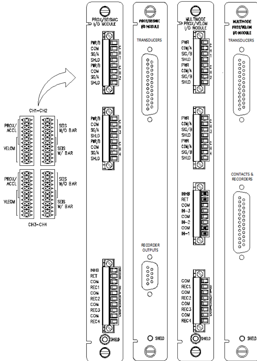
Figure 2: Side View of I/O Modules
