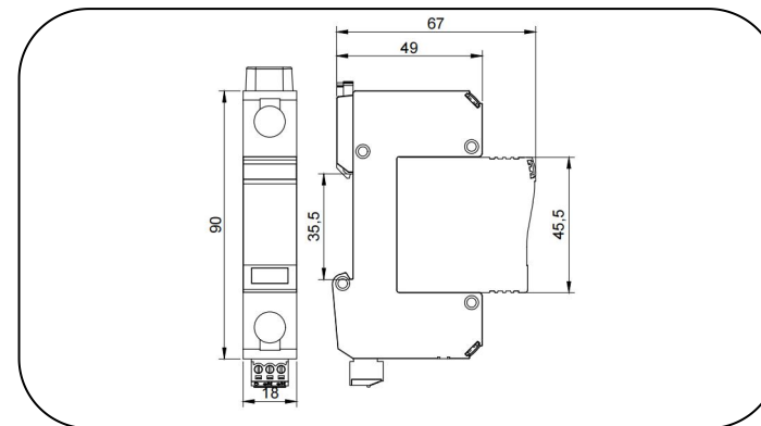
Dimension drawing
